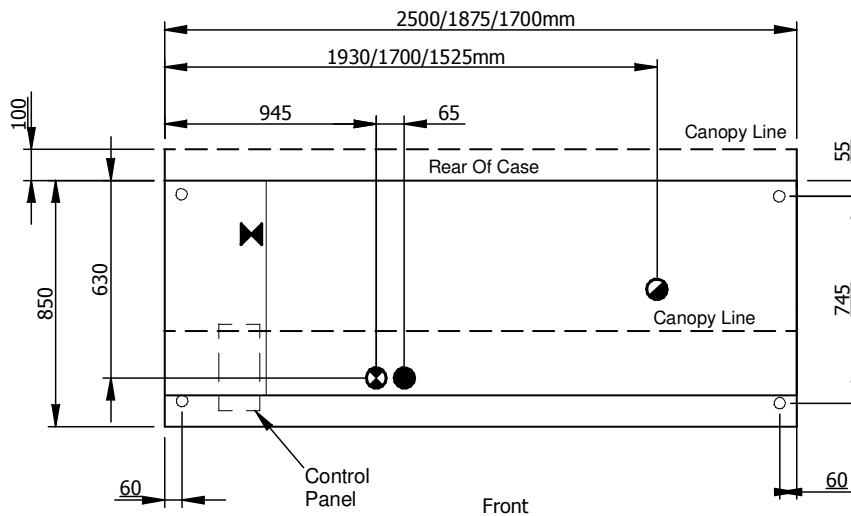
Plan of Base
